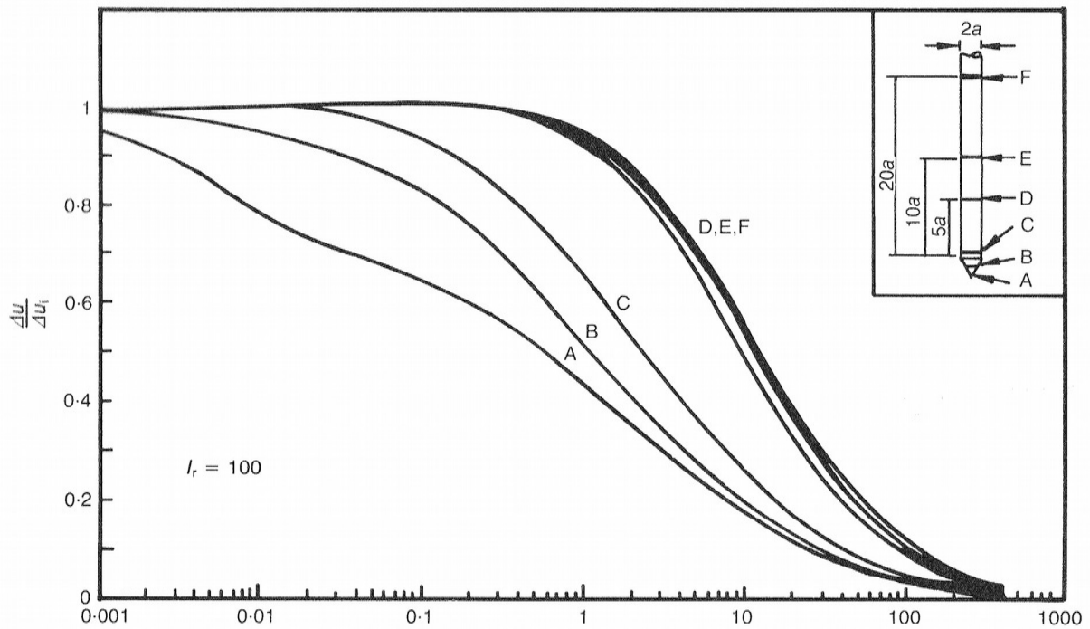
Fig. 18. Dissipation curves at different locations of a 60° cone penetrometer
