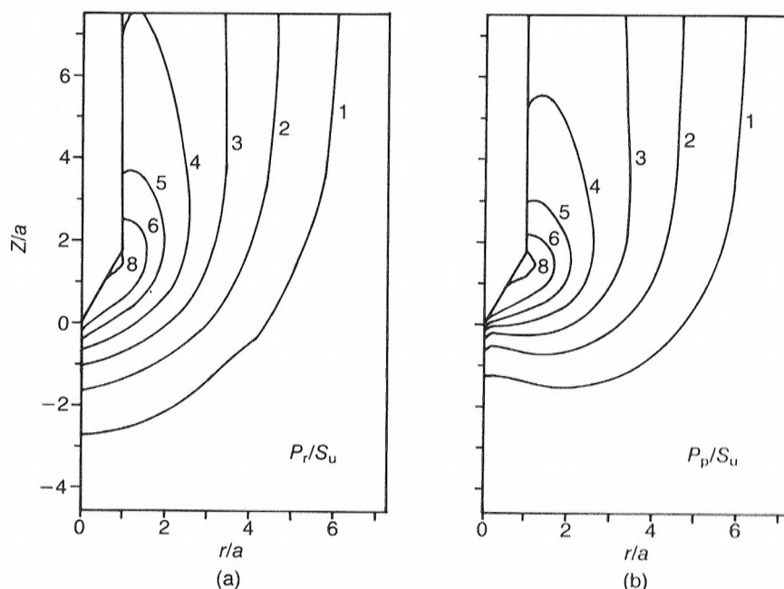
Fig. 6. Normalized mean pressure contour evaluated using (a) radial equilibrium equation and (b) Poisson's equation
