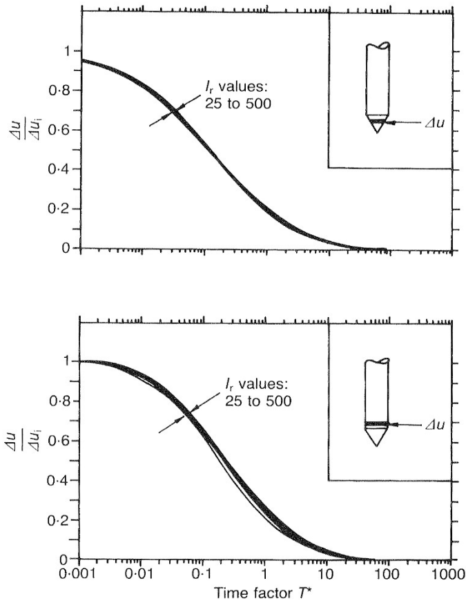
Fig. 19. Normalized dissipation curves plotted against T^*
