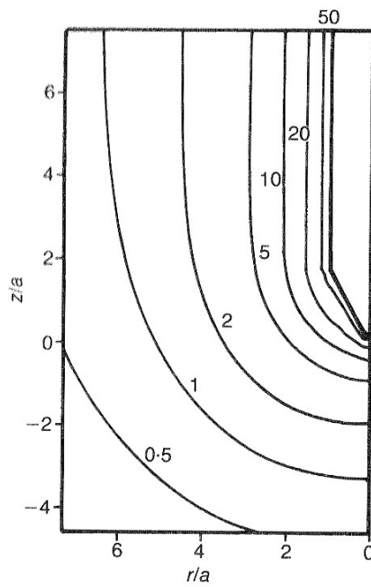
Fig. 4. Contours of \gamma_{oct}(\%) around a 60^\circ cone penetrometer
