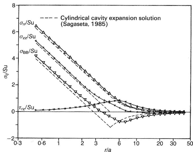
Fig. 5. Variation of stresses with radial distance on a horizontal plane at mid cone ( \beta = 10^\circ , I_r = 100 )
