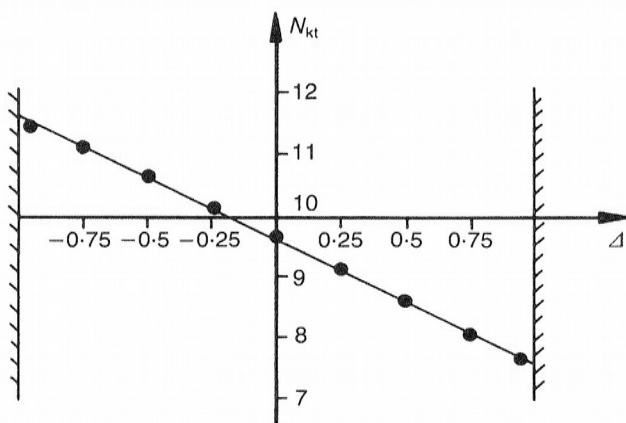
Fig. 11. Variation of N_{kt} with \Delta derived from strain path method
