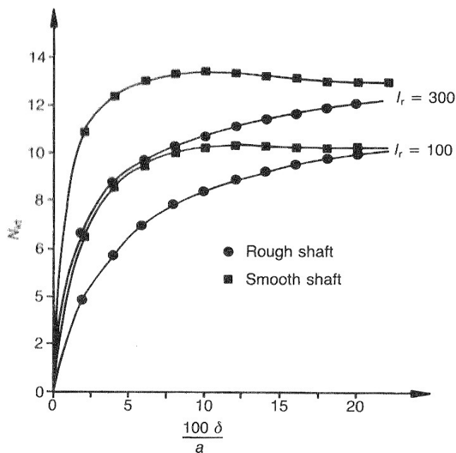
Fig. 15. Effect of shaft roughness on cone factor N_{kt}
