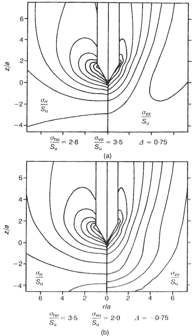
Fig. 10. Normalized stress contours for different initial stress states ( \beta = 60^\circ )
