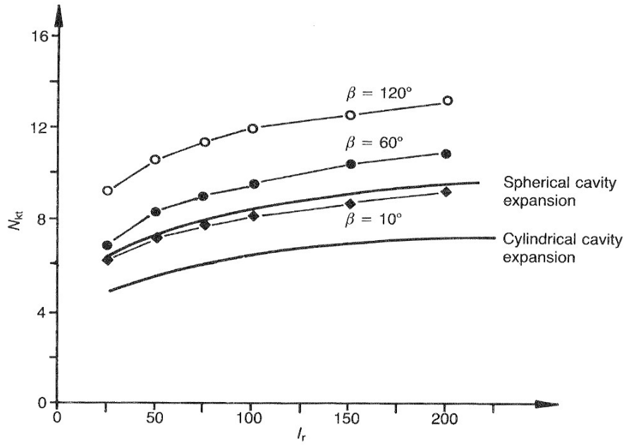
Fig. 9. Variation of N_{kt} with I_r based on strain path method
