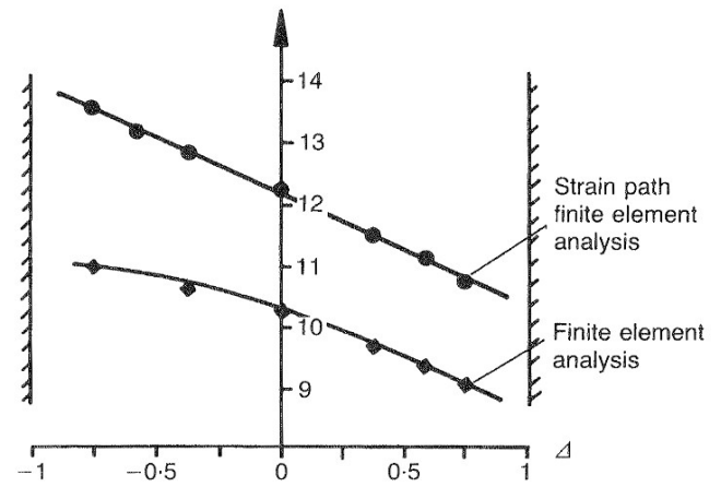
Fig. 14. Variation of N_{kt} with \Delta derived from finite element calculations
