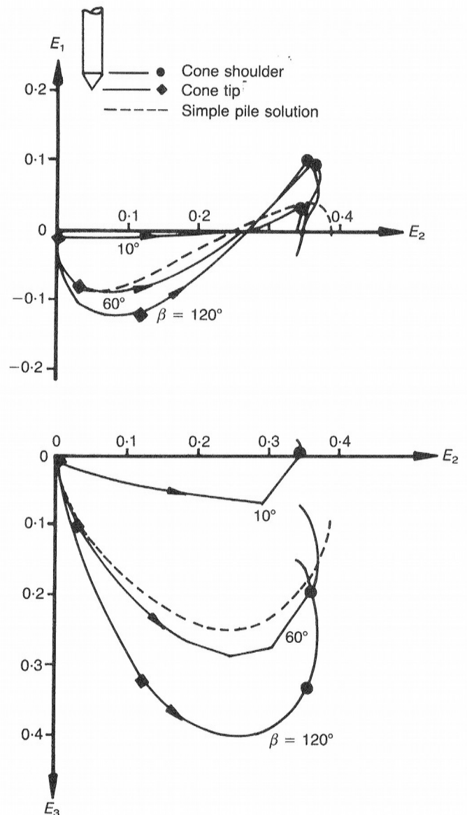
Fig. 2. Strain paths due to cone penetration
