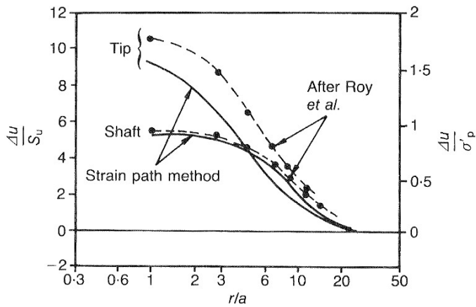
Fig. 16. Excess pore water pressure due to deep penetration
