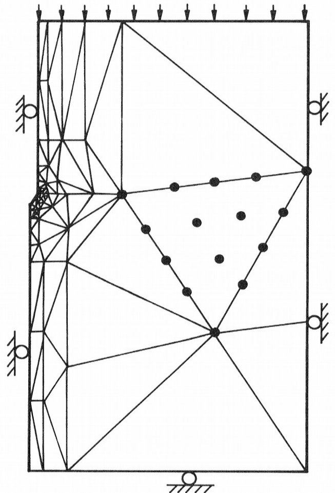
Fig. 12. Fifteen-noded finite element mesh
