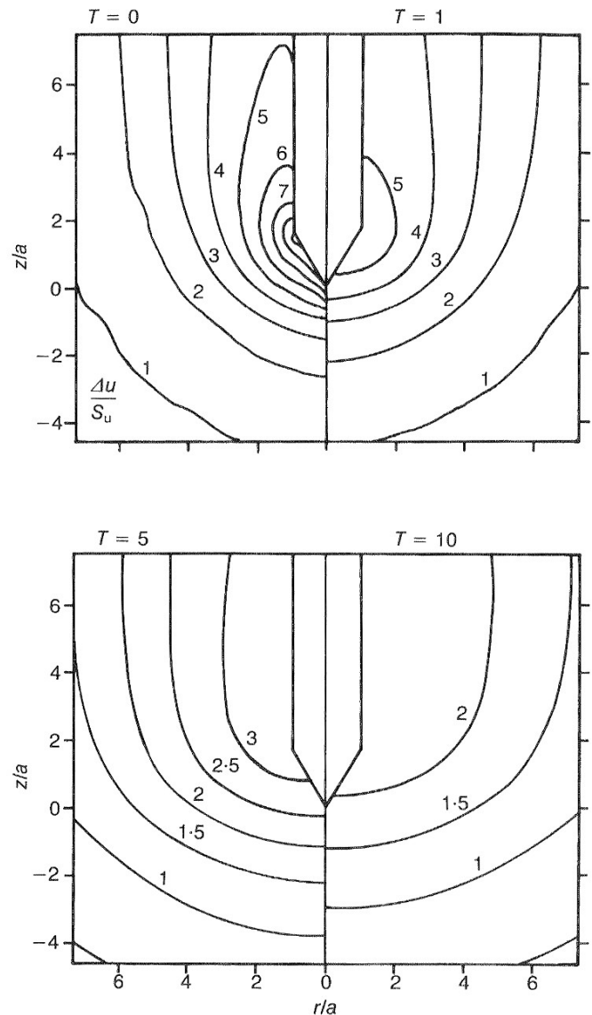
Fig. 17. Distribution of pore water pressure at various stages of dissipation
