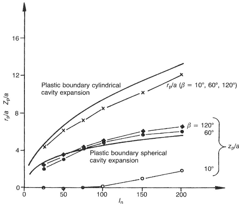
Fig. 7. Location of the elasto-plastic boundary in cone penetration
