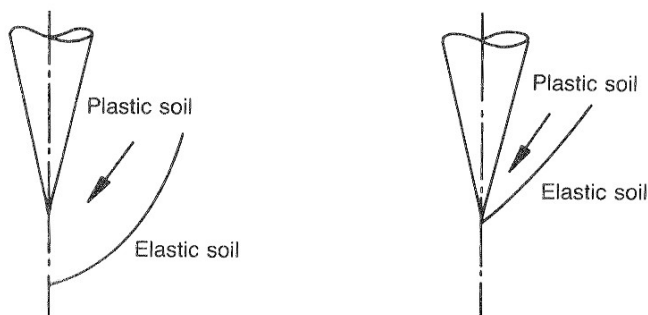
Fig. 8. Possible soil states around penetrometer tip
