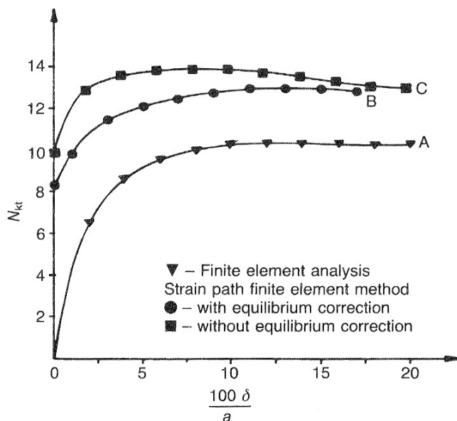
Fig. 13. Variation of N_{kt} with cone displacements
