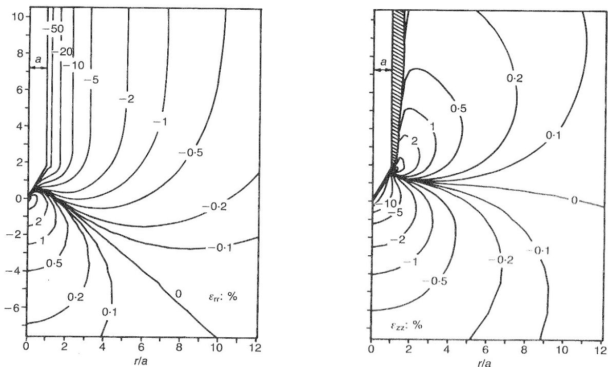
Fig. 3. Radial and axial strain contours around a 60^\circ penetrometer
