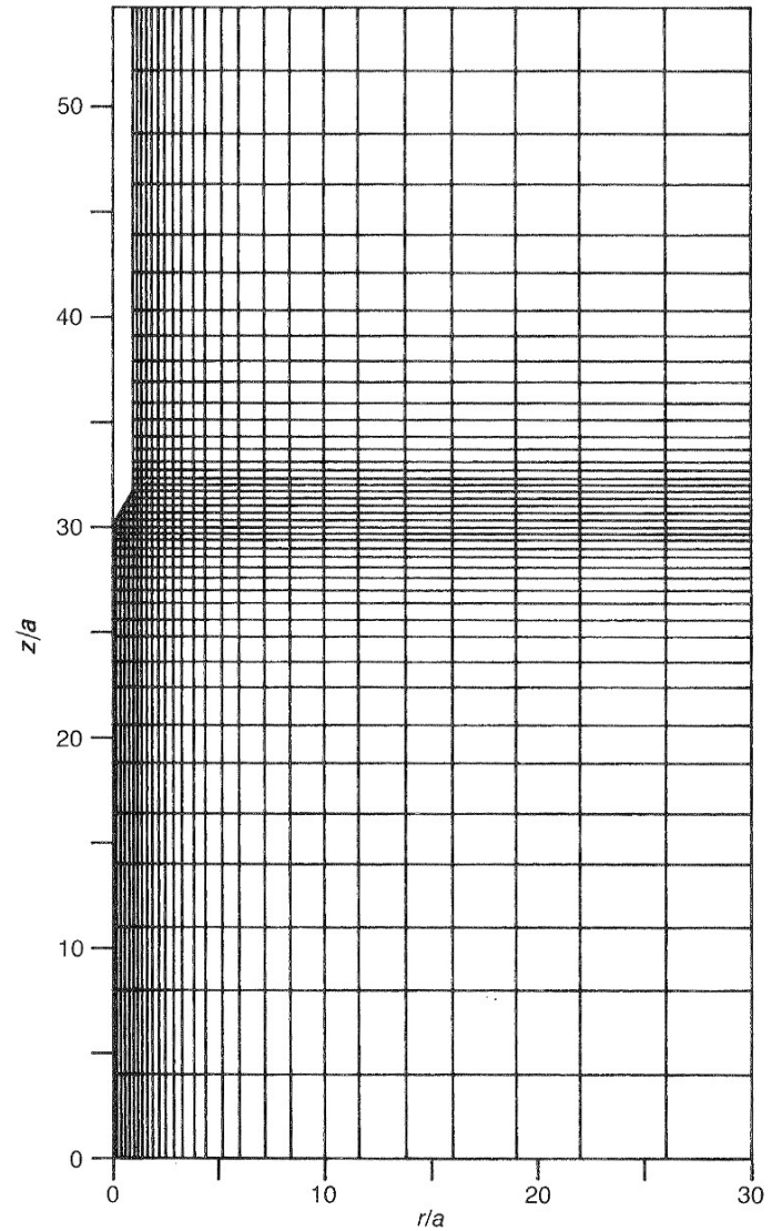
Fig. 1. Finite difference mesh for strain path analysis
