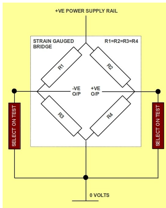
Figure 31-1 A typical transducer circuit with strain gauged bridge
